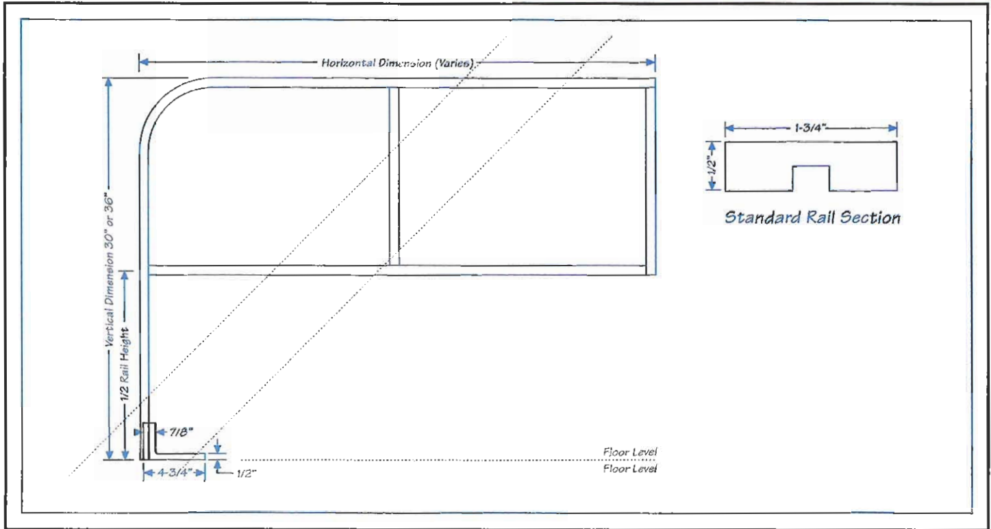
DLIW Double Line "I Brace" Wall Mounted Guide Rail
