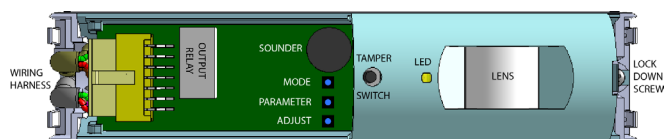
FIGURE 1 - COMPONENT LOCATIONS
